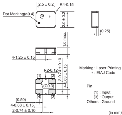
SAFSE1G88KC0T00
